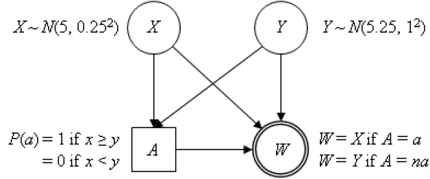
Figure 4: The revised BN for the max deterministic function
