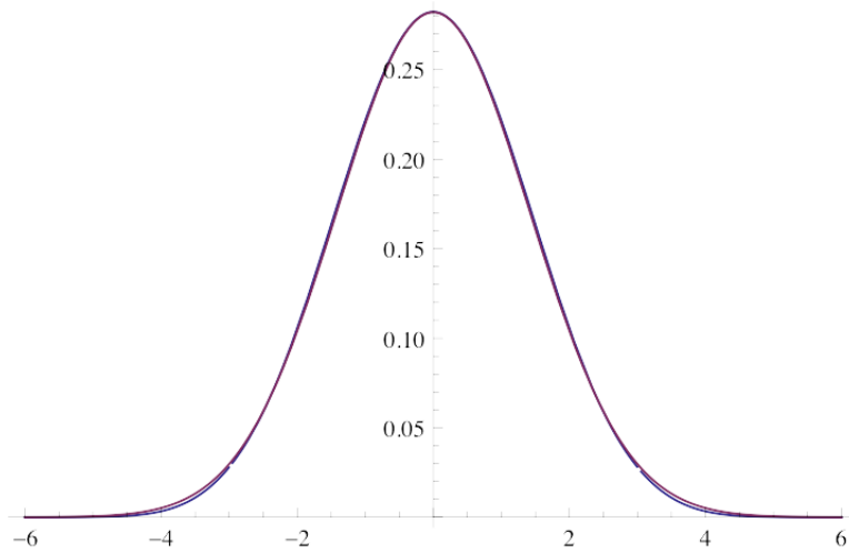
Figure 5: A graph of h_2(y) (in red) overlaid on the graph of f_Y(y) (in blue)
