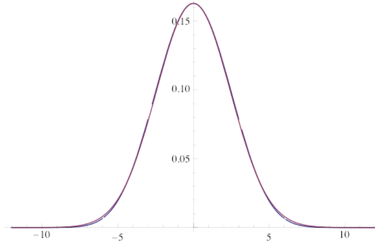
Figure 8: A graph of h_6(x) (in red) overlaid on the graph of f_X(x) (in blue)
