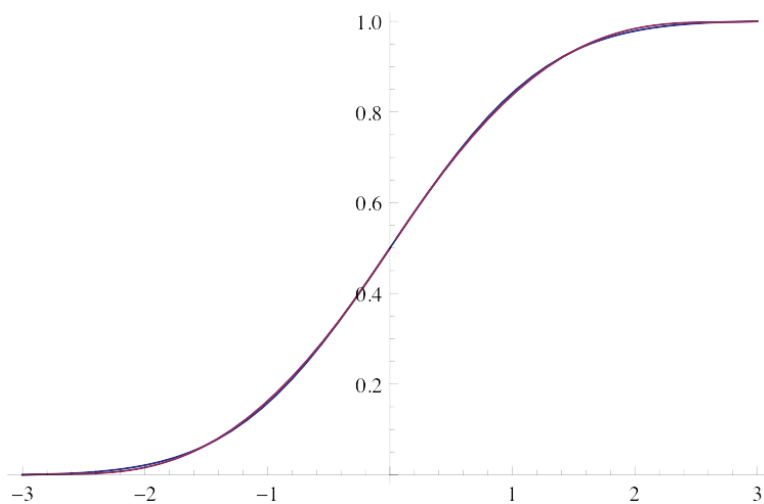
Figure 1: A graph of the CDF corresponding to g_1(z) (in red) overlaid on the graph of the CDF corresponding to \varphi(z) (in blue)
