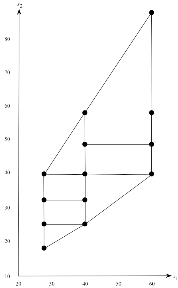
Figure 11: The region over which a MOP approximation of S_2|s_1 is computed
