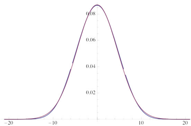
Figure 10: A graph of h_8(v) (in red) overlaid on the graph of f_V(v) (in blue)
