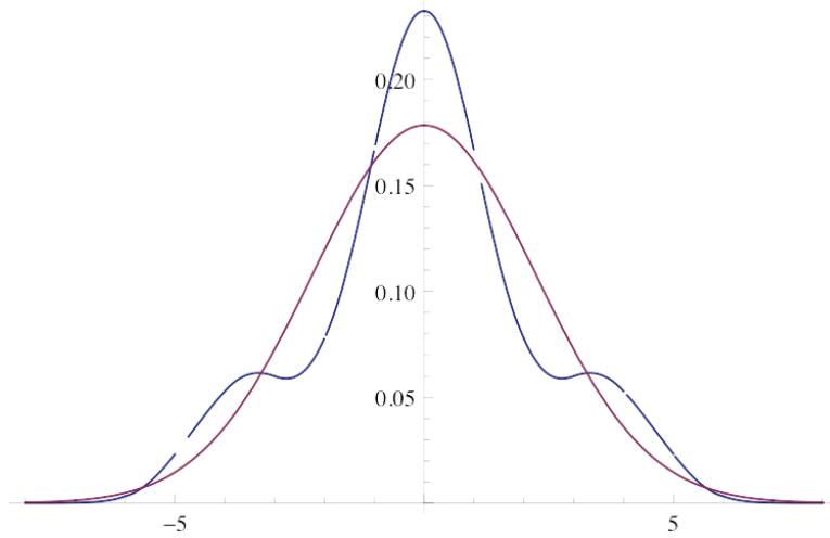
Figure 17: A graph of t_3(w) (in blue) overlaid on the graph of f_W(w) (in red)
