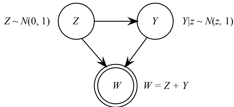
Figure 6: A Bayesian network with a sum deterministic conditional
