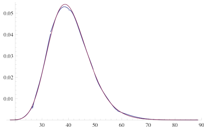
Figure 13: A plot of g_4 (in blue) overlaid on the plot of f_{S_2} (in red)
