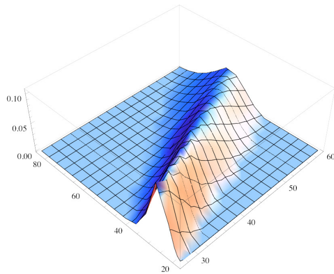
Figure 12: A three-dimensional plot of g_3(s_1, s_2)
