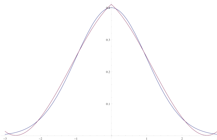
Figure 2: A graph of g_1(z) (in red) overlaid on the graph of \varphi(z) (in blue)
