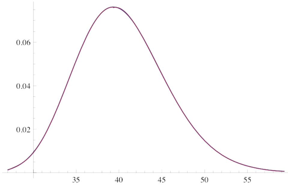
Figure 3: A graph of g_2(\cdot) (in red) overlaid on the graph of f_{S_1}(\cdot) (in blue)
