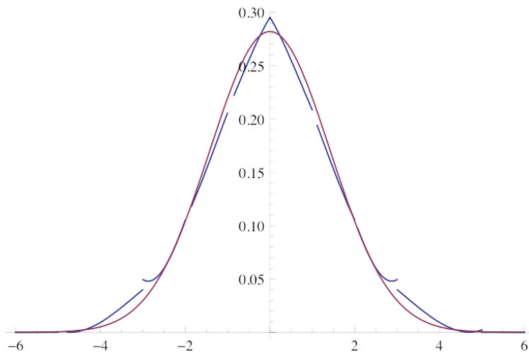
Figure 16: A graph of t_2(y) (in blue) overlaid on the graph of f_Y(y) (in red)
