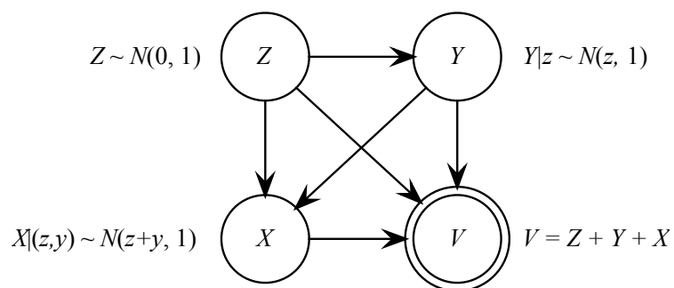
Figure 9: A Bayesian network with a three-dimensional conditional PDF
