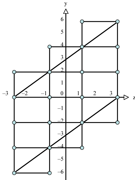
Figure 14: A graph of the domain of the MOP approximation of Y|z
