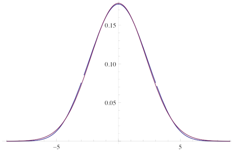
Figure 7: A graph of h_3(w) (in red) overlaid on the graph of f_W(w) (in blue)
