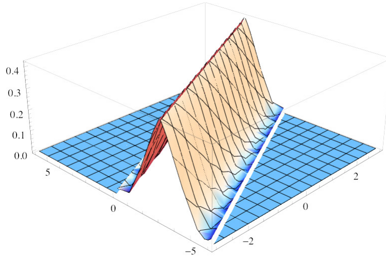
Figure 4: A three-dimensional plot of h_1(z, y)
