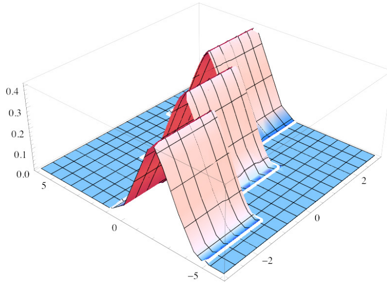
Figure 15: A three-dimensional plot of t_1(z, y)
