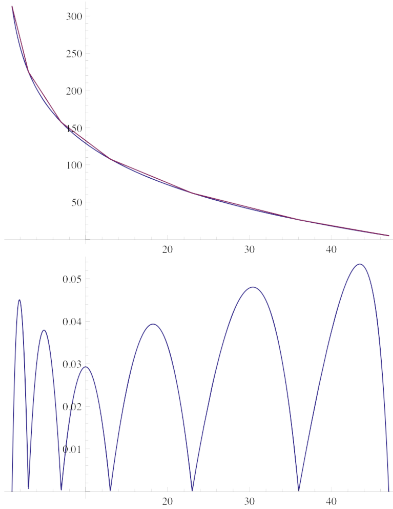
Figure 4: A Graph of f_{pQ_n}(p) (in red) Overlaid on f_{Q_n}(p) (in blue); the Bottom Graph Shows the Difference f_{pQ_n}(p) - f_{Q_n}(p) in the Curves
