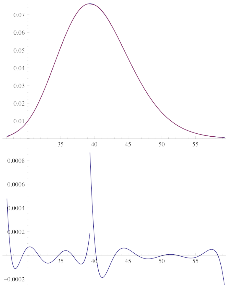
Figure 3: A Graph of \phi_{p1} (in red) Overlaid on \phi_1 (in blue); the Bottom Graph Shows the Difference \phi_1 - \phi_{p1} in the Curves
