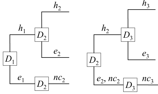
Figure 7: Constraints on D_2 and D_3
