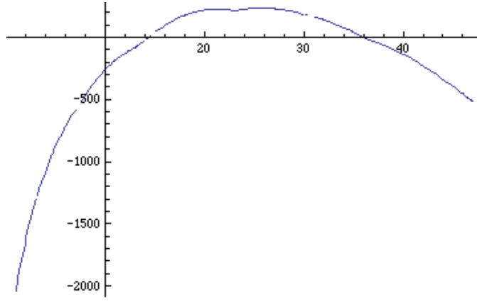
Figure 5: A Graph of \pi_6(p) vs. p
