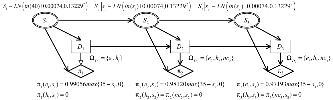
Figure 6: An ID Representation of the American Put Option
