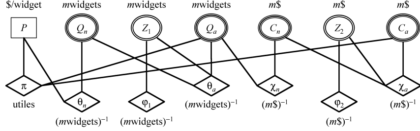
Figure 2: A VN Representation of the Entrepreneur's Problem
