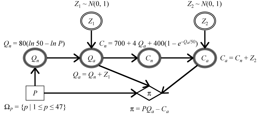
Figure 1: An Influence Diagram Representation of the Entrepreneur's Problem
