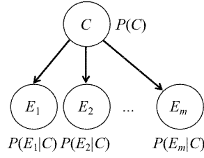
Figure 2: A NB Model as a Bayesian Network
