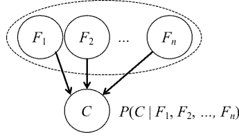
Figure 1: A LR Model as a Bayesian Network
