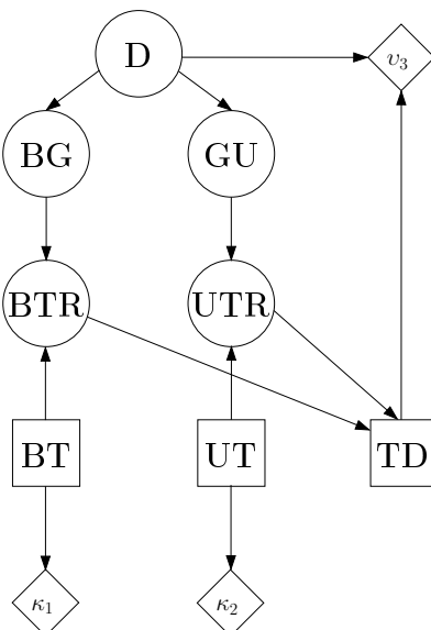
Figure 10: An unconstrained ID model for the diabetes diagnosis problem
