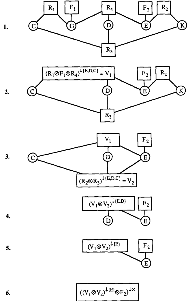
Figure 2. The fusion algorithm applied to the valuation network of Figure 1 using deletion sequence GKCD E.
