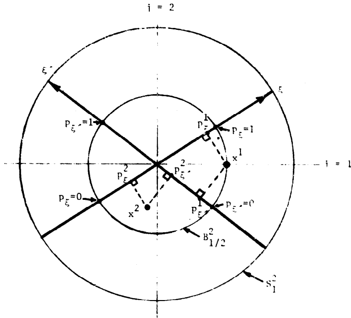
Fig. 2. Issues, voter profiles and the corresponding probabilities for each voter on each issue.
