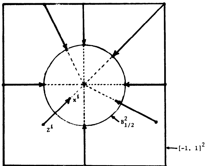
Fig. 1. The mapping f: [-1, 1]^2 \longrightarrow B_{1/2}^2 .
