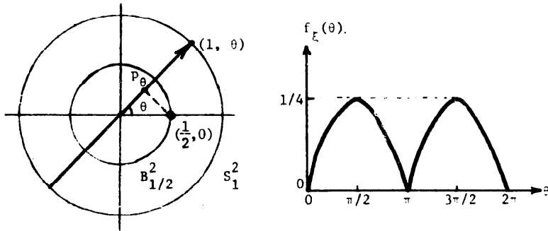
Fig. 3. The probability p_\theta and the distribution f_\xi(\theta) .
