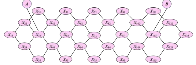
Figure 5: The Communication Network undirected graphical model. The variable X_{ij} is in the i^{th} column ( i = 1, \dots, 13 ), and j^{th} row ( j = 1, \dots, 5 ).
