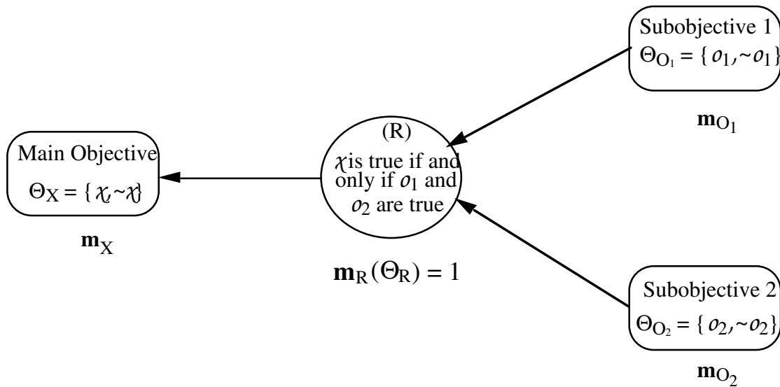
Figure 4. An AND-Tree with Three Nodes.
