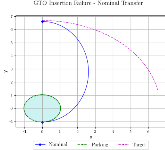
Figure 3: Nominal GTO transfer orbit and target GEO orbit.
