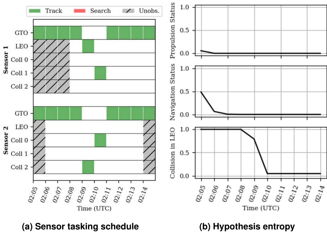
Figure 7: Case 2: navigation anomaly
