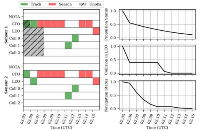
Fig. 2. Test Case: propulsion explosion, schedule and entropy
