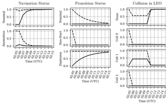
Fig. 3. Test Case: propulsion explosion, hypothesis resolutions (solid line for belief, dashed line for plausibility)
