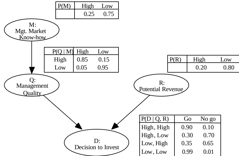
FIGURE 2: A Bayesian Network with Conditional Probability Tables
