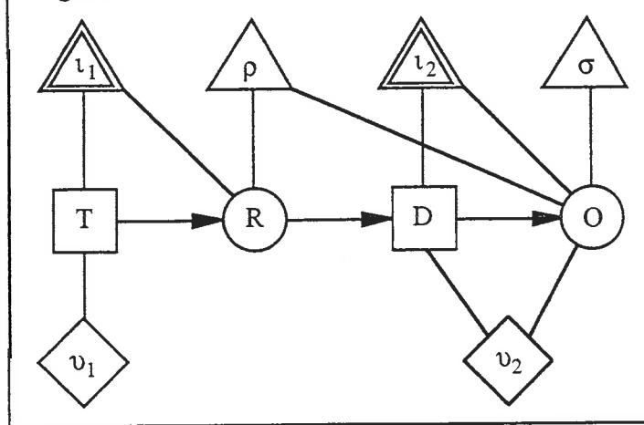
Figure 2. A valuation network for the OW problem.
