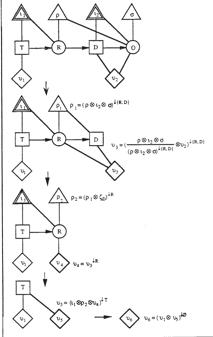
Figure 3. The fusion algorithm for the OW problem.
