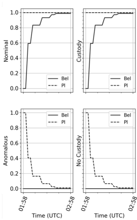
Figure 8: GOES 14 Belief and Plausibility vs. Time
