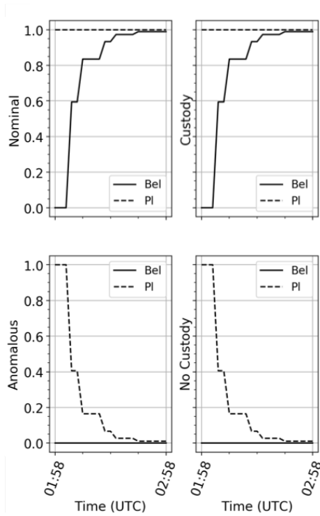
Figure 9: ANIK G1 Belief and Plausibility vs. Time
