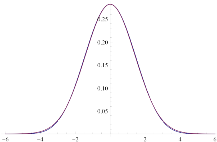
Figure 5: A graph of h_2(y) (in red) overlaid on the graph of f_Y(y) (in blue)
